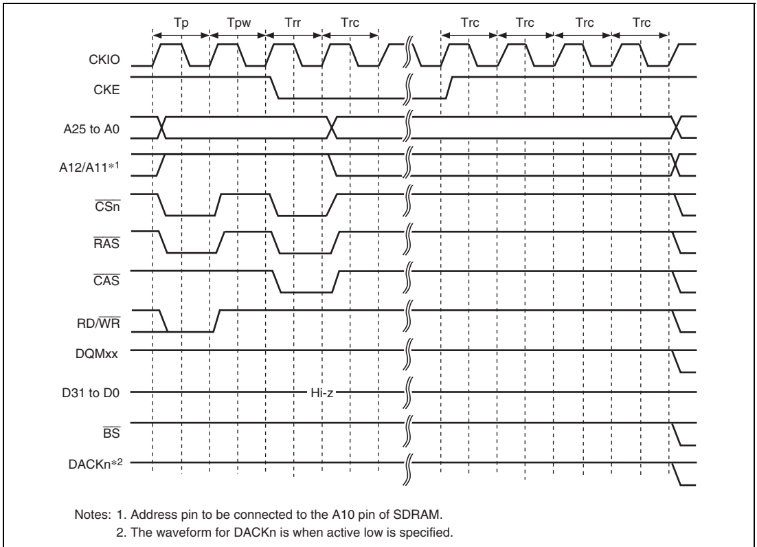
Figure 9.26 Self-Refresh Timing
